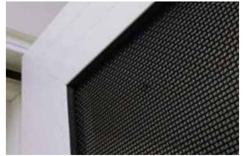
Mesh panels are secured in product frames with patented mechanical attachment systems
